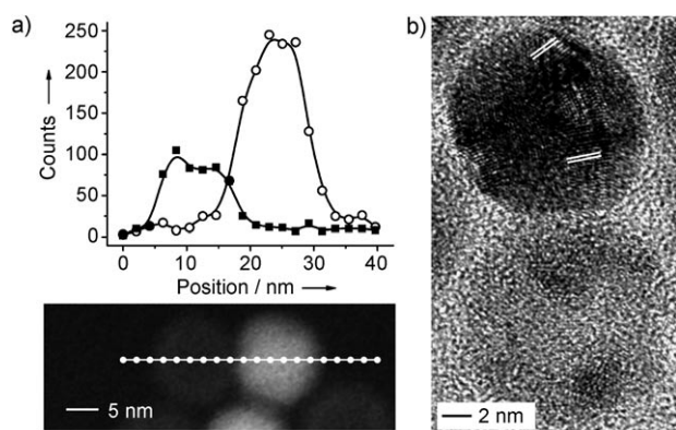
Figure 3. Characterization of \text{Ag-Fe}_x\text{O}_y dumbbell-like nanoparticles formed at 600 s with a) high-resolution line-scan EDS analysis of Ag ( \circ ) and Fe ( \blacksquare ), and b) HRTEM. The line and dots in the high-angle annular dark-field scanning transmission electron microscopy (HAADF-STEM) image (bottom frame in (a)) show the scanning path and the corresponding examining positions. The adjacent lattice fringes in (b) are measured to be 0.238 nm that matches well with the (111) interplanar distance of fcc Ag.
